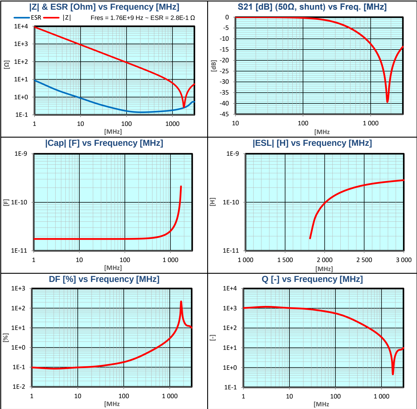
Electrical Characteristics
