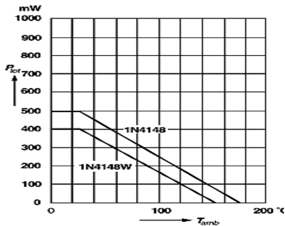
Fig 2: Admissible Power Dissipation Versus Ambient Temperature
