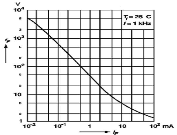
Fig 3: Dynamic Forward Resistance Versus Forward Current
