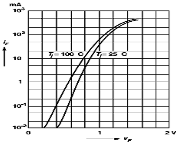
Fig 1: Forward Characteristics
