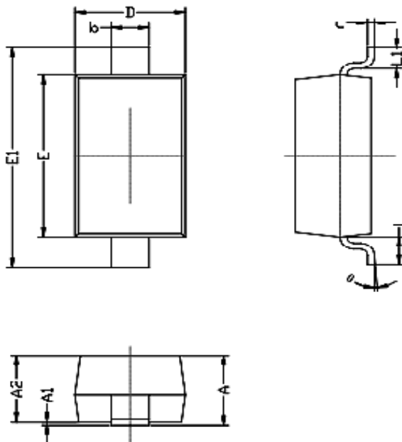
Package SOD123GW
