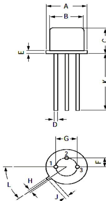
TO-39 Metal Can Package
