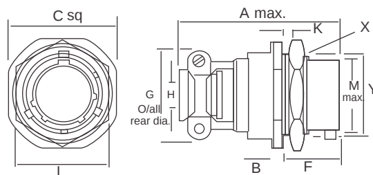
62 IN - 14F Single hole mounting with grommet and grommet nut fitted with integral strain relief clamp has panel 'O' ring seal
