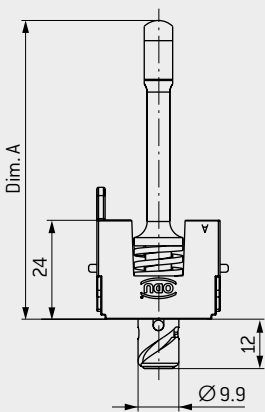
SPINDLE 1 – 12 mm (180°)
