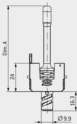
SPINDLE 3 – 16.3 mm (360°)
