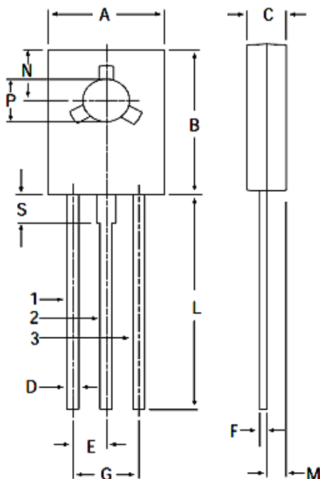
TO-186 Leaded Plastic Package
