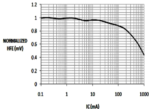
Fig 4: Normalized hFE vs Collector Current
