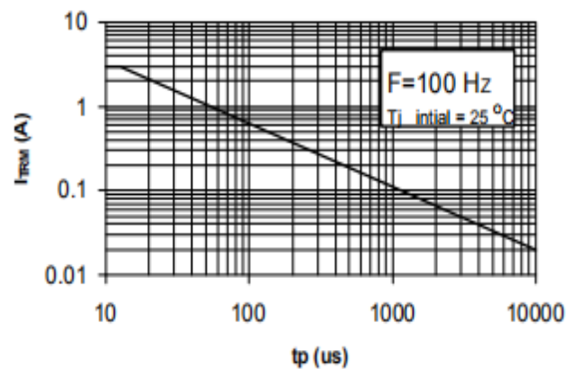
Figure 5: Peak pulse current versus pulse duration (maximum value)
