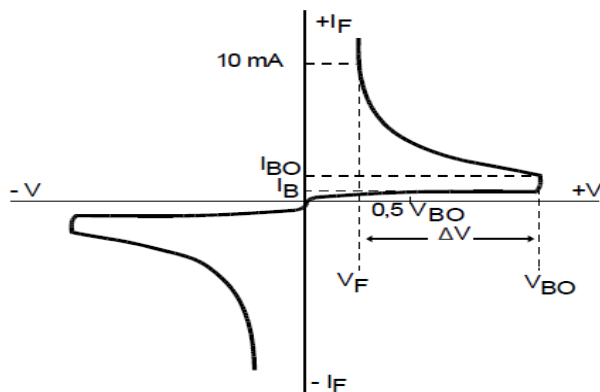
Figure 1. Voltage - current characteristic curve.
