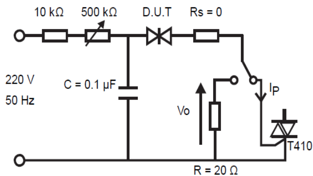
Figure 2. Rise time measurement
