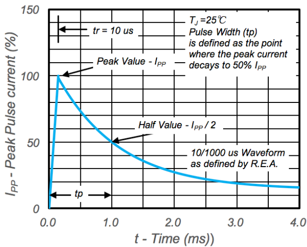
FIG.3 – Pulse Waveform
