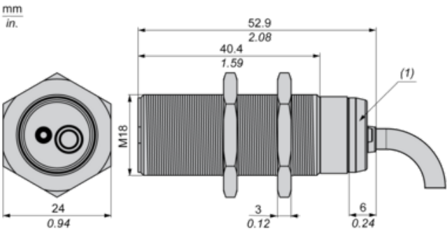
(1) LED
